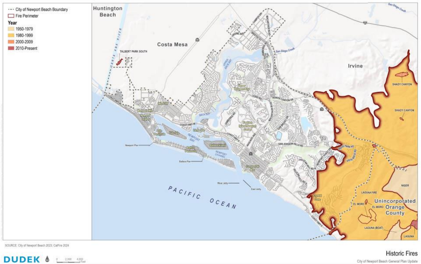
Figure 7. Historic Fires
