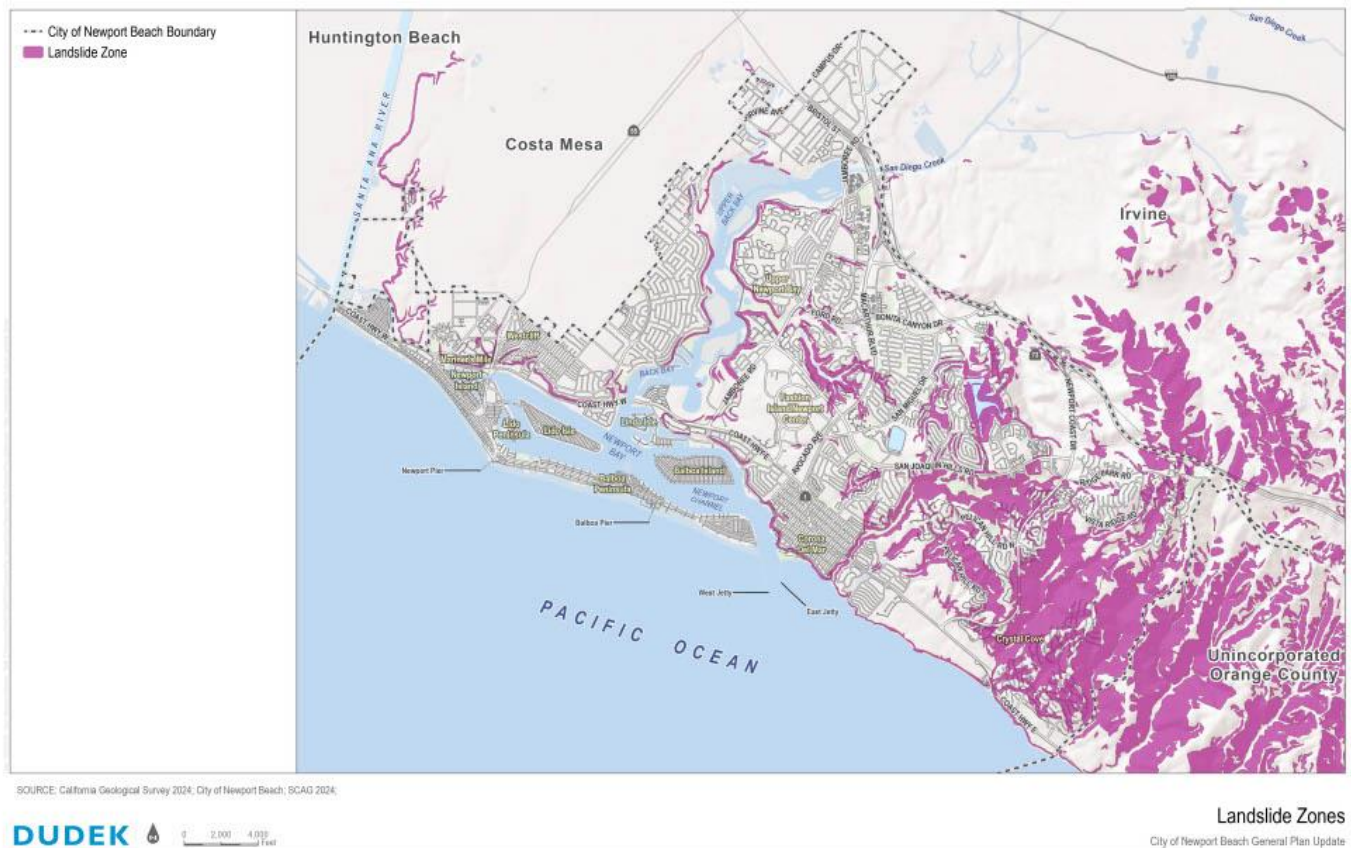
Figure 3. Landslide Zones
