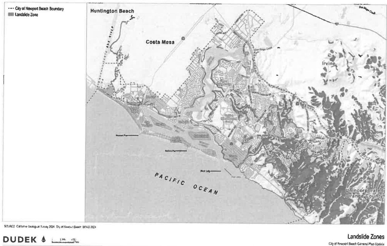
Figure 3. Landslide Zones
