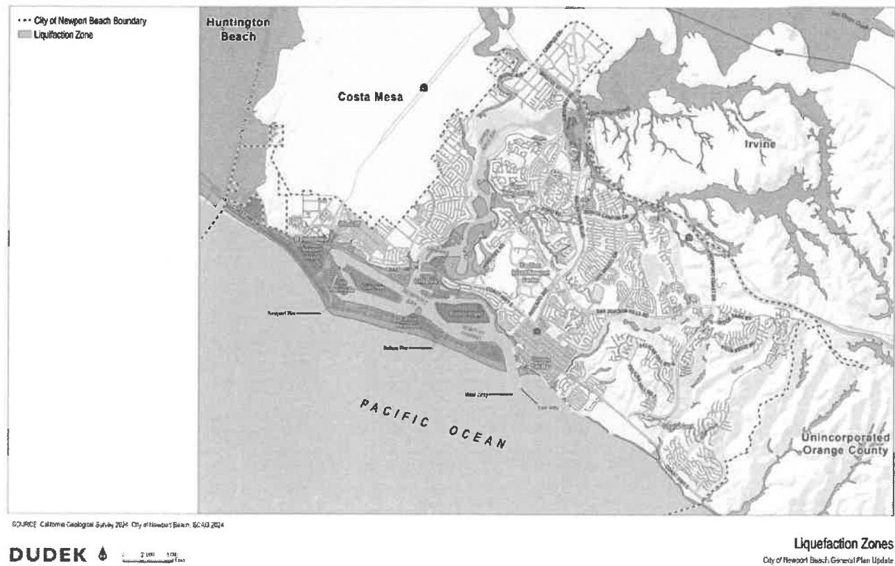
Figure 4. Liquefaction Zones
