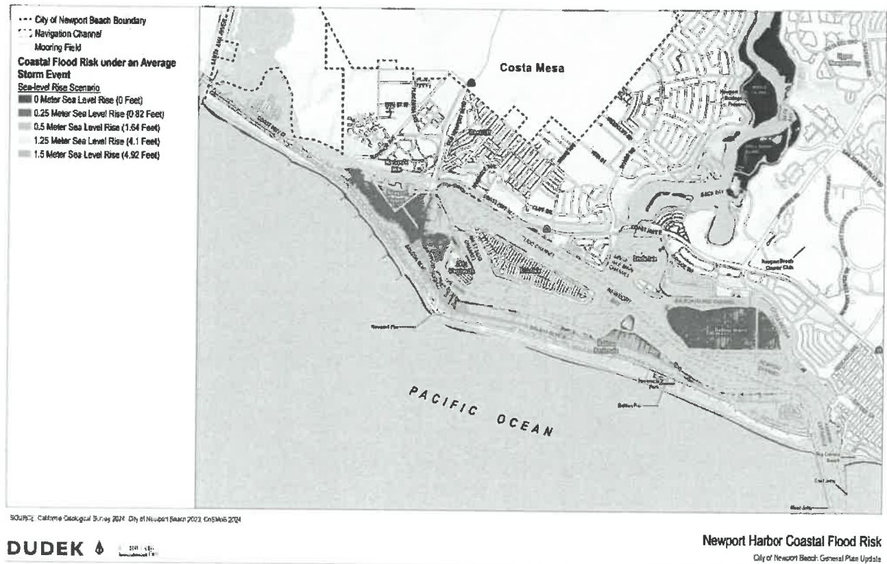
Figure 2. Newport Harbor Coastal Flood Risk
