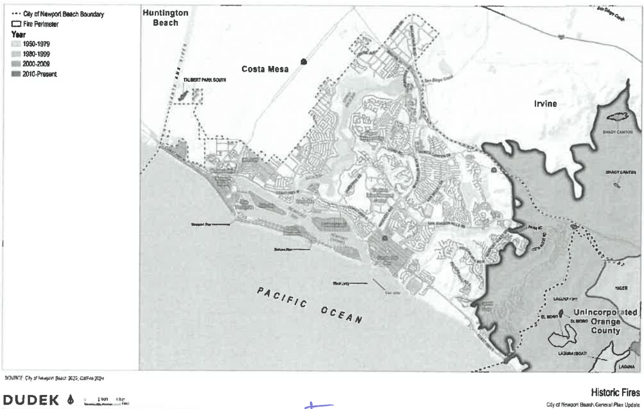
Figure 7. Historic Fires
